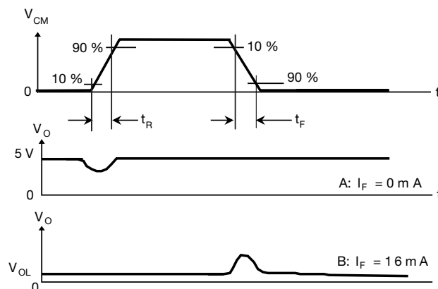
Fig. 6 - Measurement Waveform of CMR
